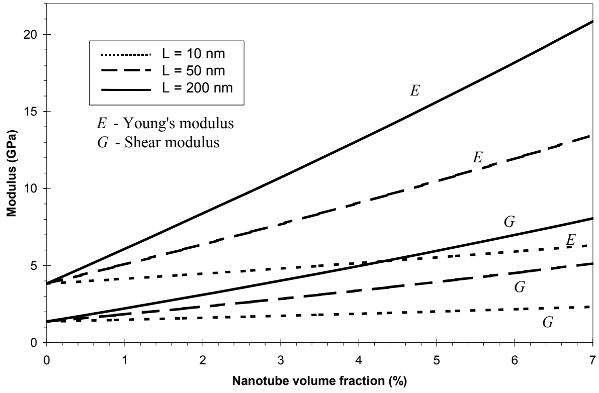
FIG. 8. Modulus of random SWNT/LaRC-SI composite material vs. nanotube volume fraction
